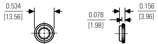
3/8 - 32 Panel Nut Bright Nickel
