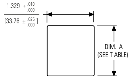
Mounting Detail
