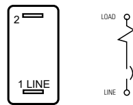
Shunt Trip Single Pole
