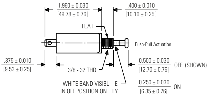
Push-Pull, Single Pole
