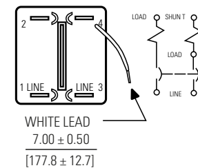
Two Pole ( 1 pole relay )
