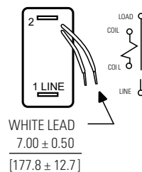
Relay Trip (Note A) Single Pole
