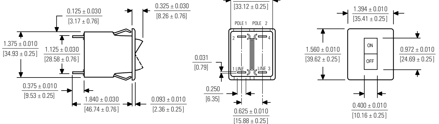
Rocker, Two Pole
