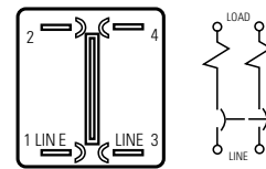
Two Pole ( 1 pole shunt )
