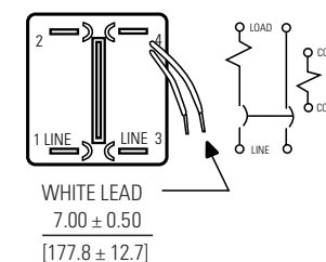
Two Pole ( 1 pole relay )
