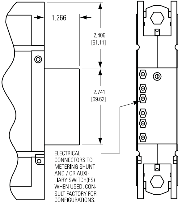
Metering Shunt
