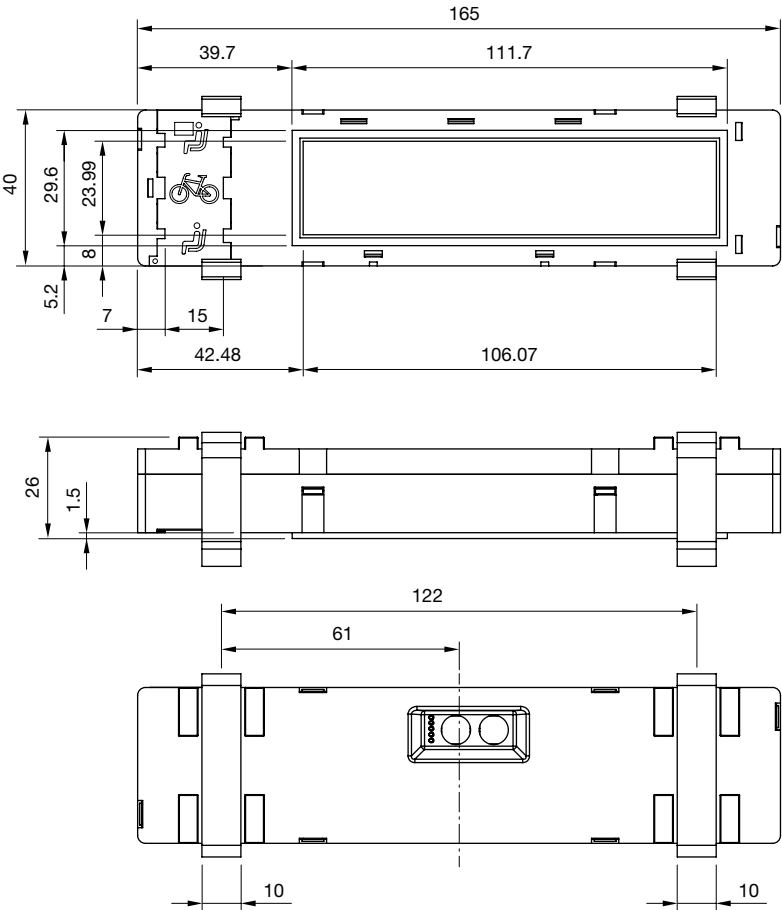
Fig. 5: Dimensions (mm) housing clip attachment.
