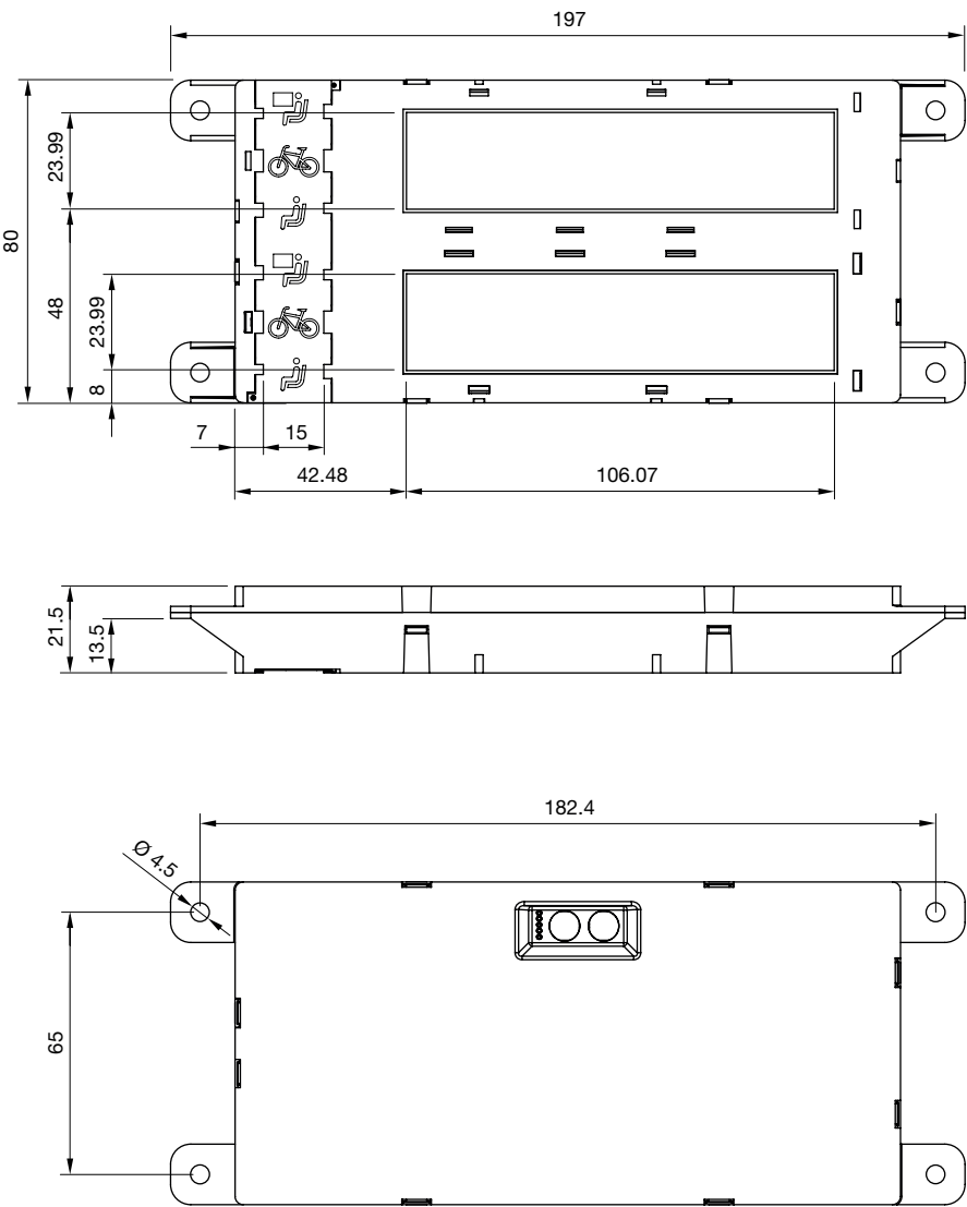
Fig. 7: Dimensions (mm) housing with two displays.
