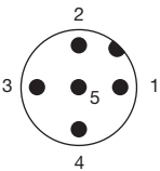
Fig. 9: Pin assignment CAN.
