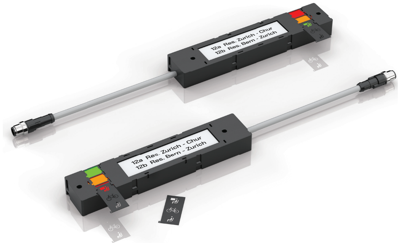
Fig. 8: Display with cable outlet left and right, with M12 connector as an example.
