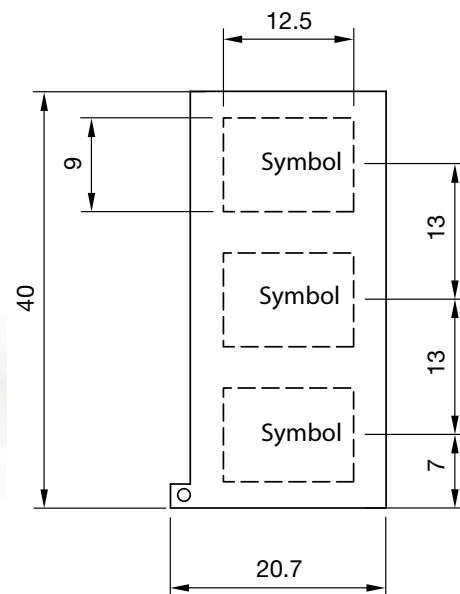
Fig. 4: Dimensions (mm) insert strip.
