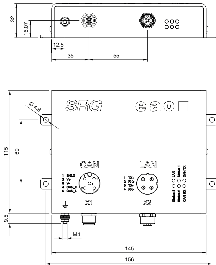
Fig. 11: Dimensions (mm) housing Gateway (SRG).
