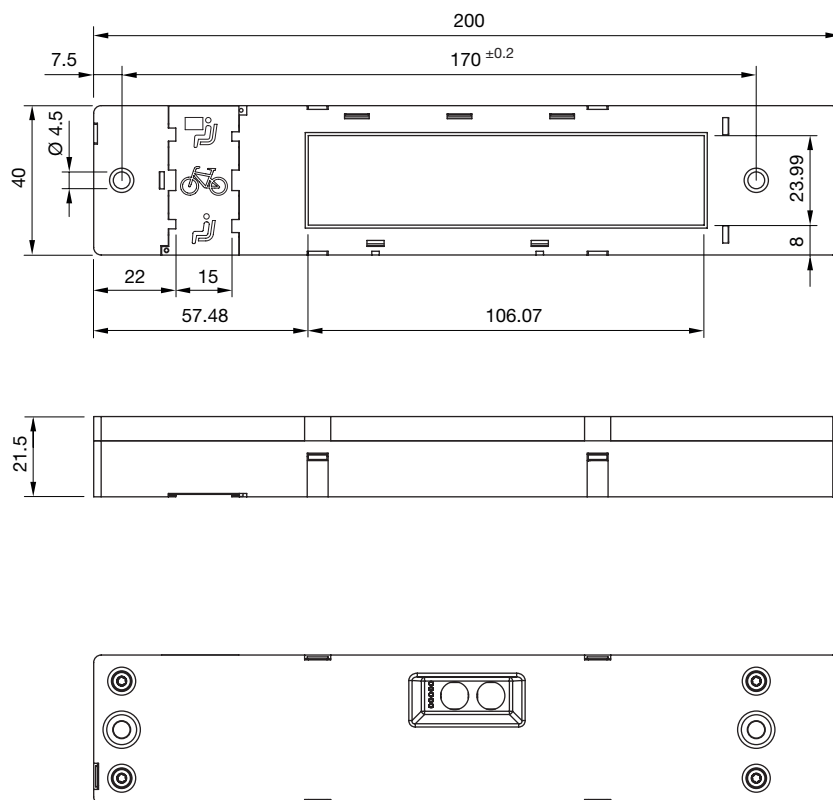
Fig. 6: Dimensions (mm) housing screw mounting.
