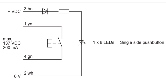
Wiring diagram 2
